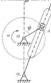
Figure 5. Schematic Diagram of Crank-Rocker Mechanism
