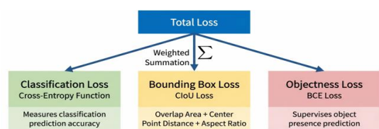
Figure 8. YOLO Loss Function Structure
