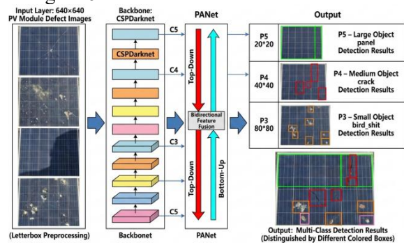
Figure 5. Flowchart of the YOLO Photovoltaic Panel Defect Detection Algorithm
